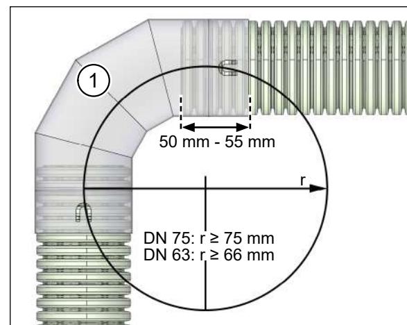
Abb. 9: Flexrohrbogen 90°
